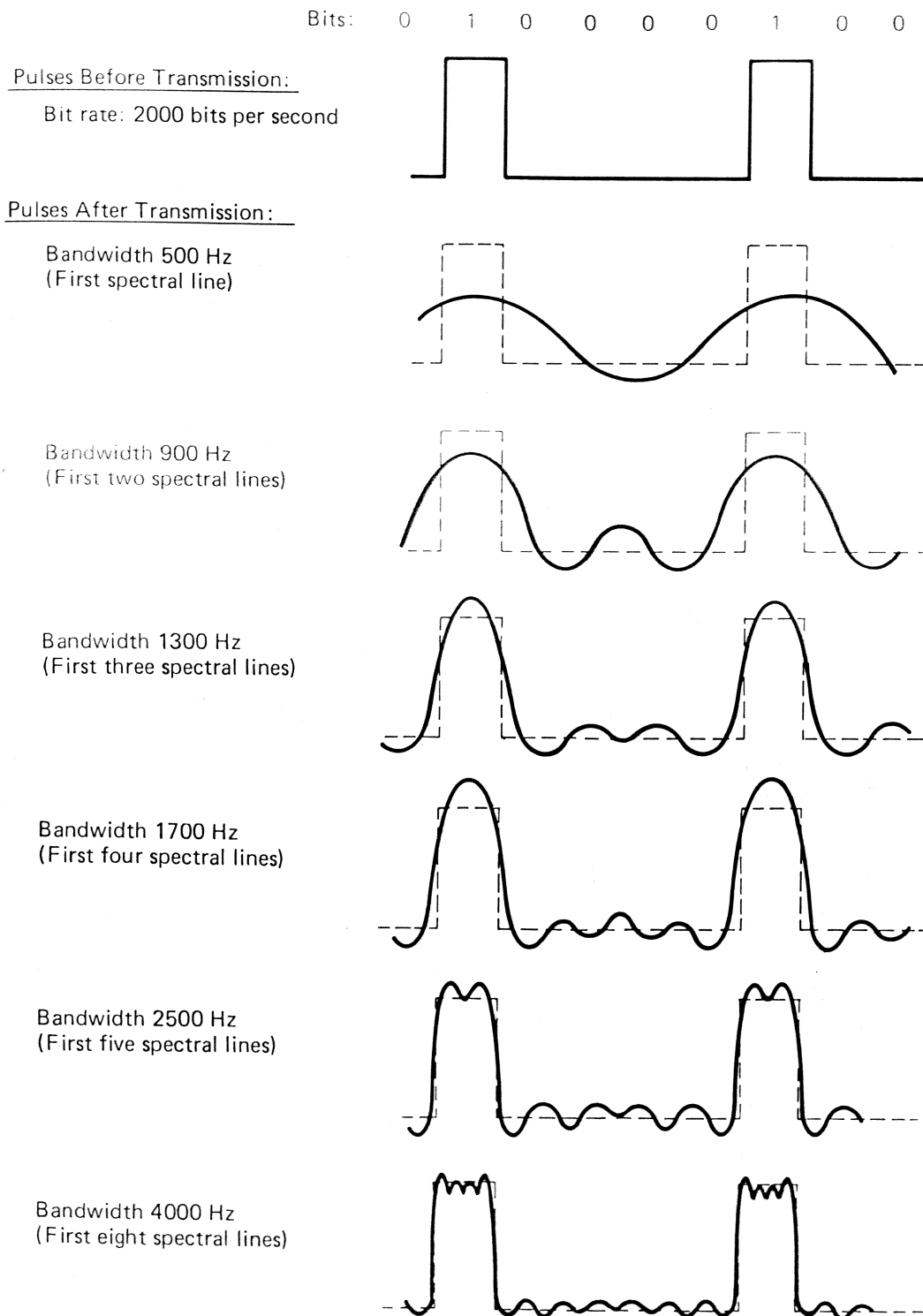
Figure 8.14 The effect of transmitting the pulses in Fig. 8.13 over differing bandwidths. Telecommunications and the Computer, by James Martin; Prentice-Hall, 1976.
